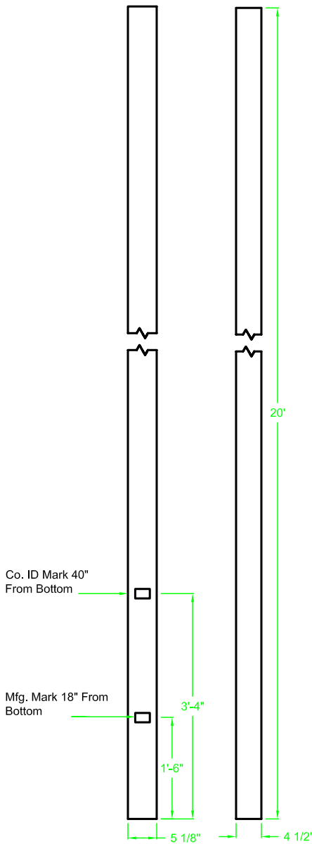
Pole Details
