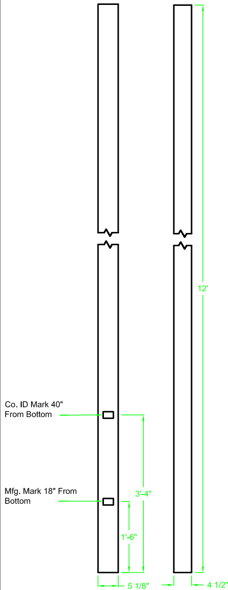
Pole Details
