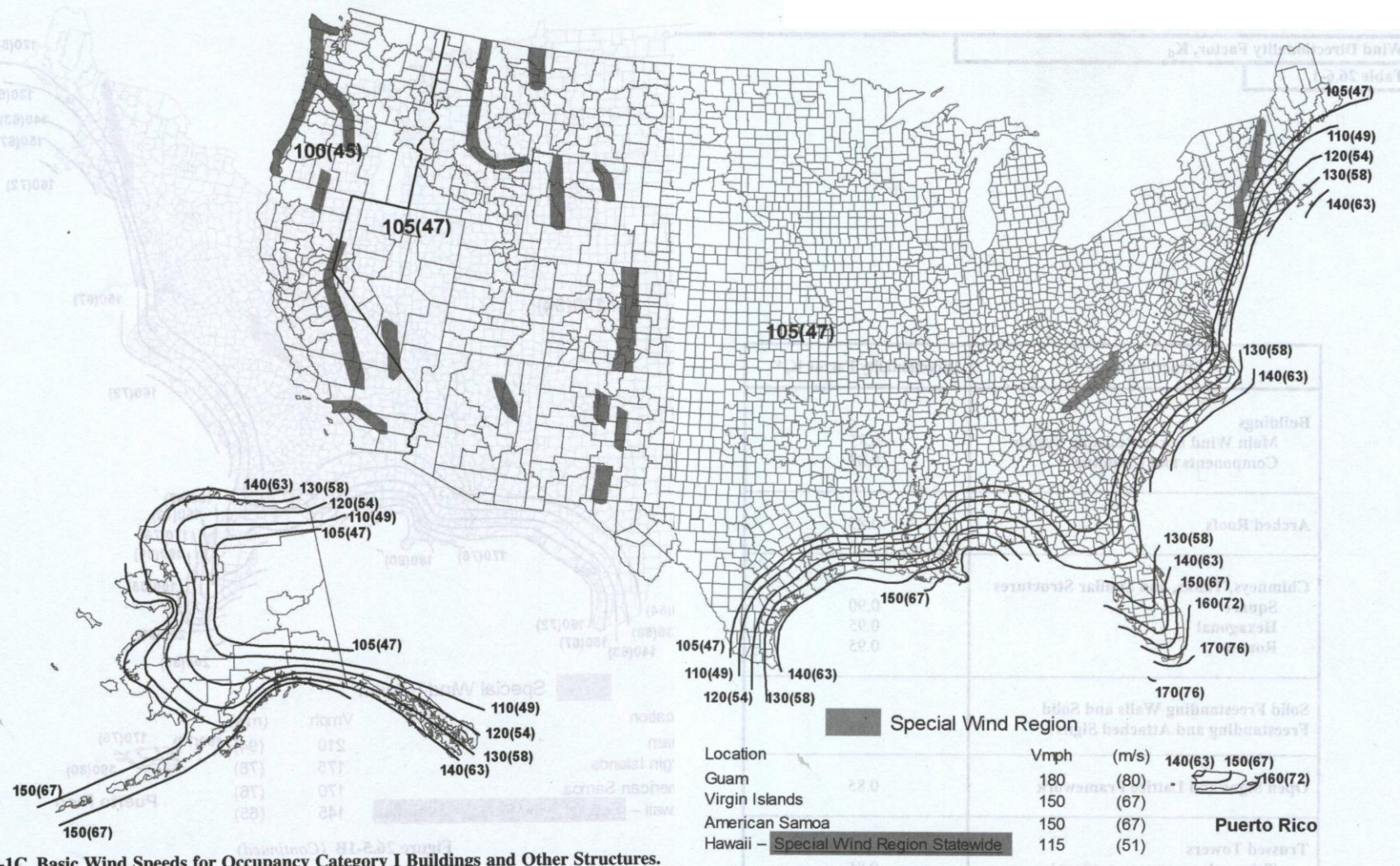
Figure 26.5-1C Basic Wind Speeds for Occupancy Category I Buildings and Other Structures.
