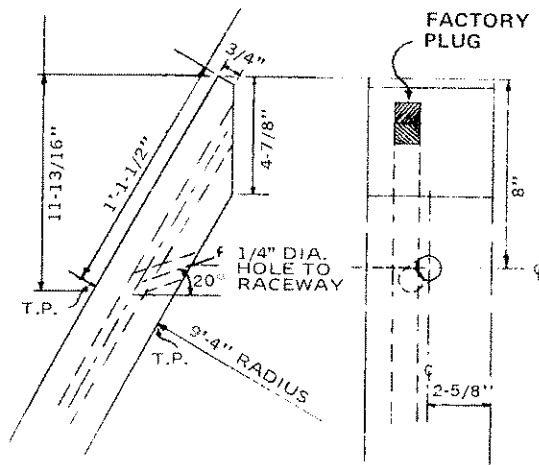
Top Framing - Detail A
