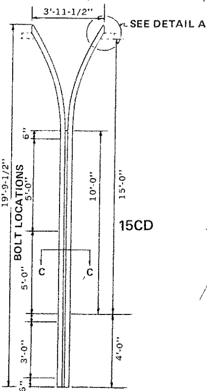
Double Curved Scale 3/16"=1'- 0"
