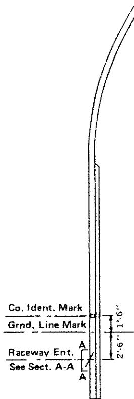
Pole Details
