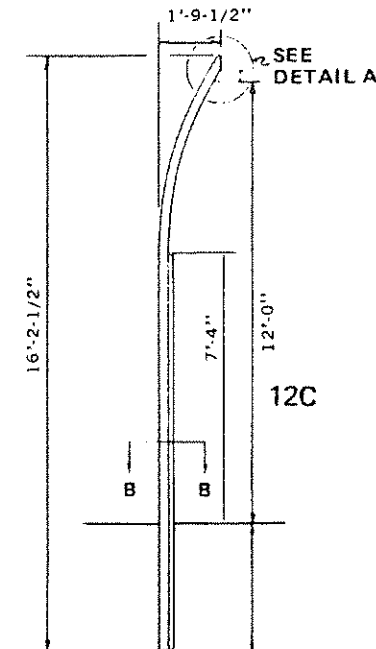
Single Curved Scale 3/16" = 1'-0"
