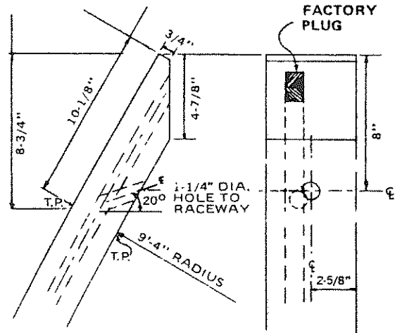
Top Framing - Detail A
